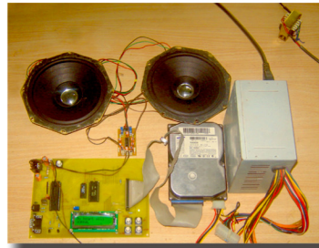
Digital Mp3/WAV Player Using Hard Disk
